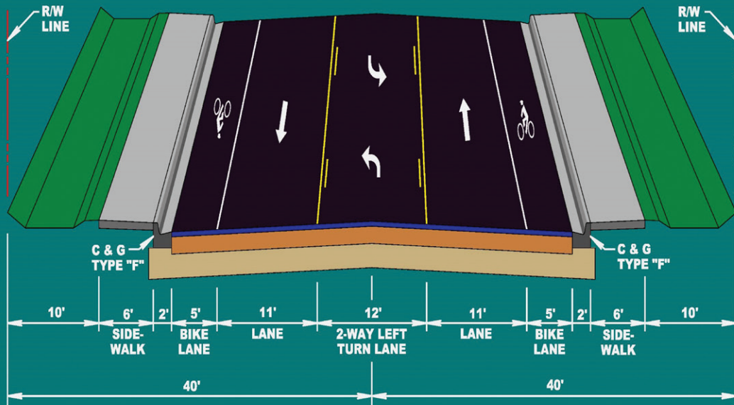
TYPICAL SECTION 80' RIGHT OF WAY SPEED LIMIT = 35 MPH
